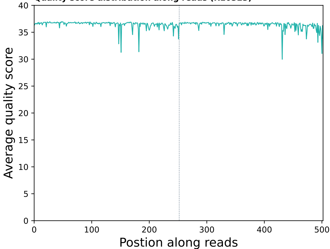
Quality score distribution along reads (R10323)
